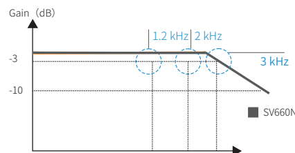
Speed loop response graph
