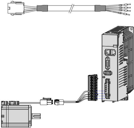
Figure 2-5 Diagram of connection between servo drive output terminals and the servo motor
